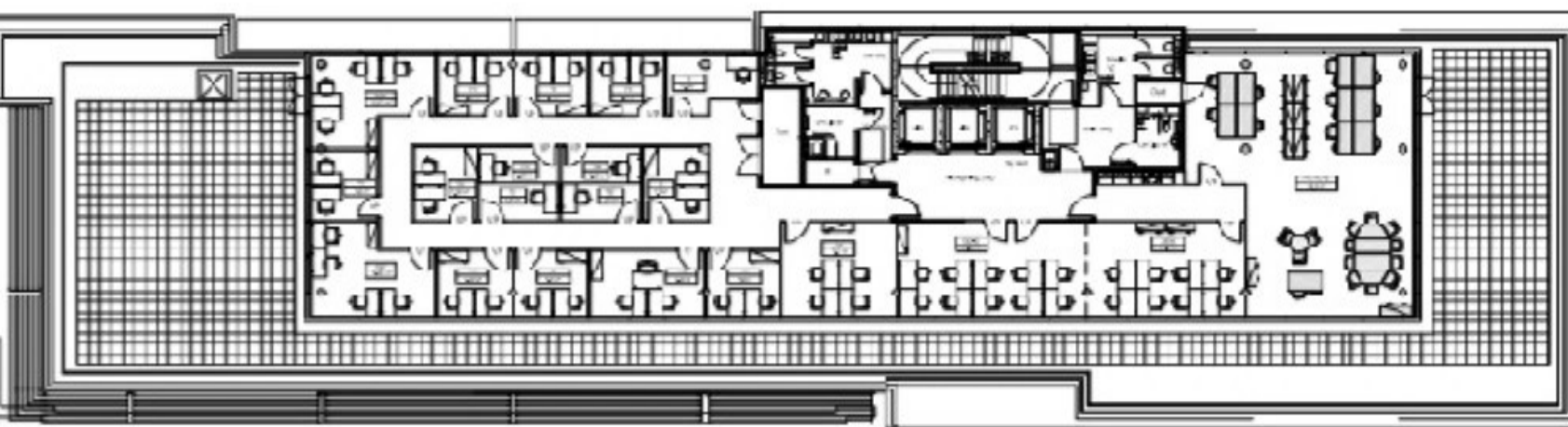
SIXTH FLOOR PLAN
